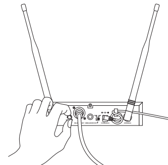
11. Adjust Gain
